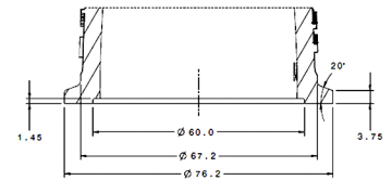
TURBINE INLET V-BAND CONNECTIONS
