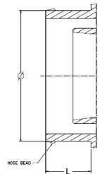
COMPRESSOR INLET HOSE CONNECTIONS Ø51.15 X 29.05
